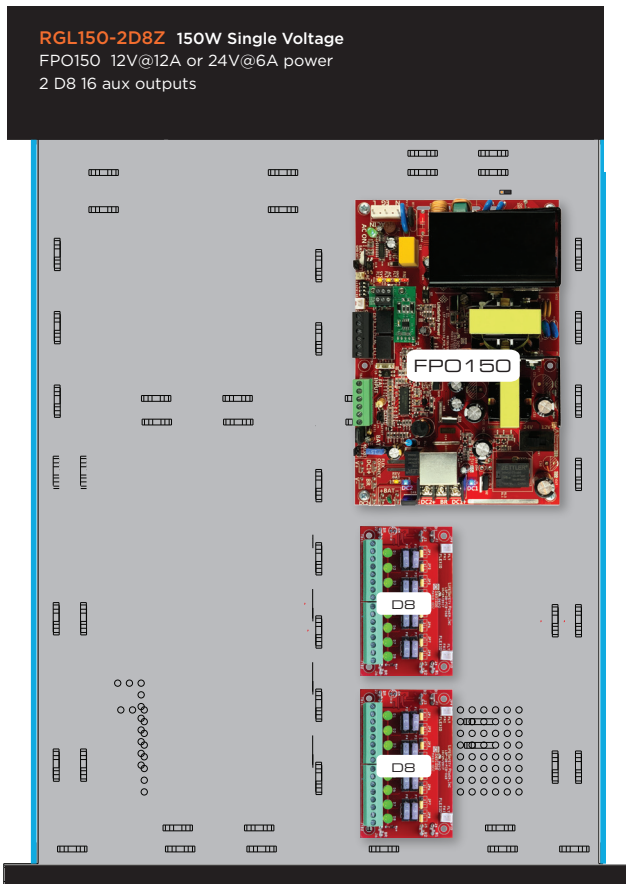
Drawer layout example of FPO150
