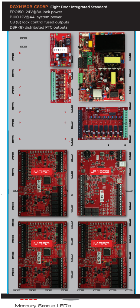
Drawer layout example of 8 door dual voltage
