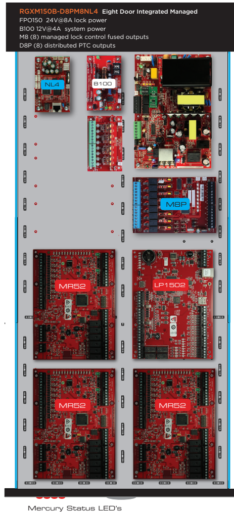
Drawer layout example of 8 door dual voltage managed system
