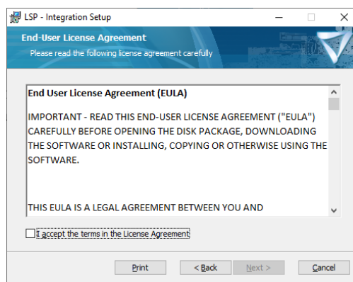
Figure 2: EULA Window
