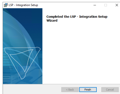
Figure 5: Installation complete
