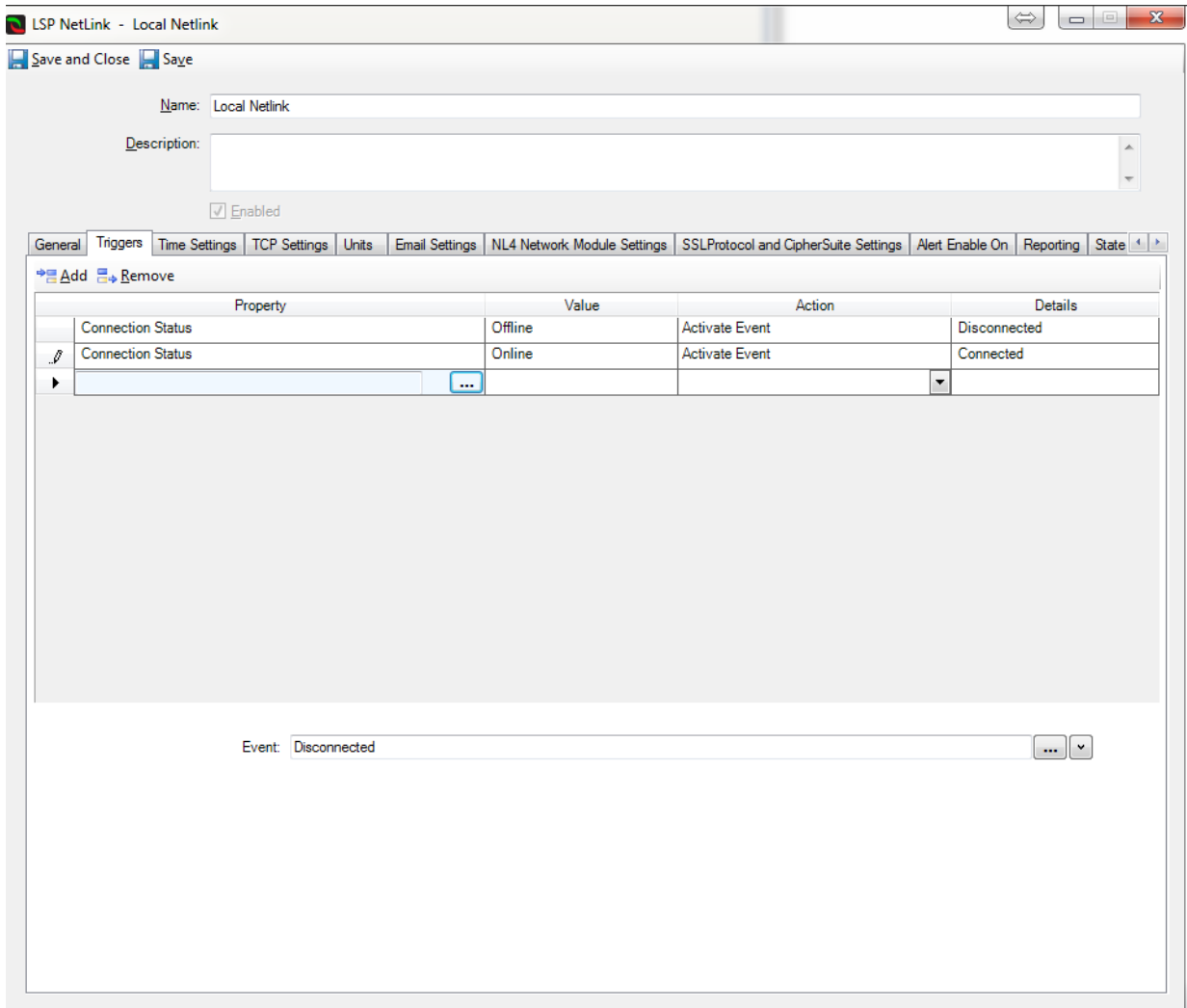
Figure 9: Triggers Tab
