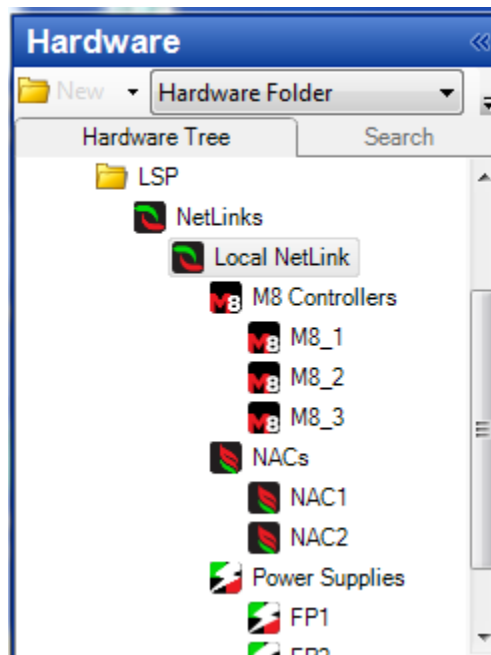
Figure 7: Hardware Tree
