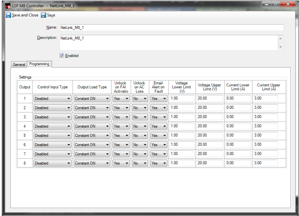
Figure 26: General Tab
