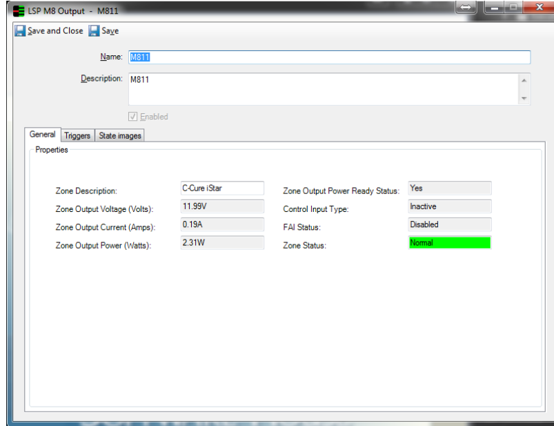
Figure 27: General Tab
