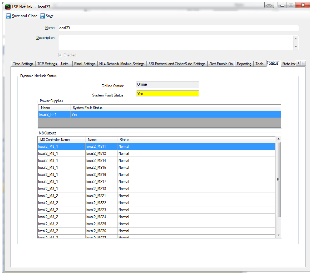
Figure 19: Status Tab
