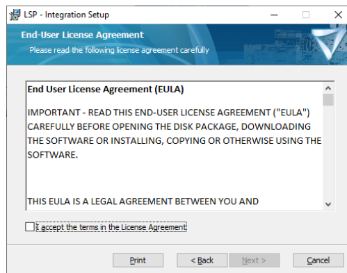
Figure 2: EULA Window
